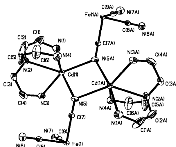
Fig. 1 ORTEP 9 plot of the \mu_3 -cyano-bridged trimetallic building-block, showing 30% probability displacement ellipsoids. The \text{Cd}(1) atom is also coordinated by another \text{N}(7) atom (2.459(4) Å) from \mu\text{-CN}^- generated by the symmetry operation (-x + 1, -y, -z + 2) . Bond lengths: \text{Cd}(1)\text{--N}(1) 2.343(5), \text{Cd}(1)\text{--N}(2) 2.653(4), \text{Cd}(1)\text{--N}(3) 2.326(5), \text{Cd}(1)\text{--N}(4) 2.336(5), \text{Cd}(1)\text{--N}(5) 2.526(4), \text{Cd}(1)\text{--N}(5A) 2.575(4), \text{Fe}(1)\text{--C}(7) 1.899(4), \text{Fe}(1)\text{--C}(8) 1.927(5), \text{Fe}(1)\text{--C}(9) 1.912(4), \text{C}(7)\text{--N}(5) 1.154(6), \text{C}(8)\text{--N}(6) 1.151(6), \text{C}(9)\text{--N}(7) 1.172(6) Å. Bond angles: \text{N}(5)\text{--Cd}(1)\text{--N}(5A) 78.00(14), \text{Cd}(1)\text{--N}(5)\text{--Cd}(1A) 102.00(14), \text{C}(7)\text{--N}(5)\text{--Cd}(1) 129.8(4), \text{N}(5)\text{--C}(7)\text{--Fe}(1) 179.1(4)°.
